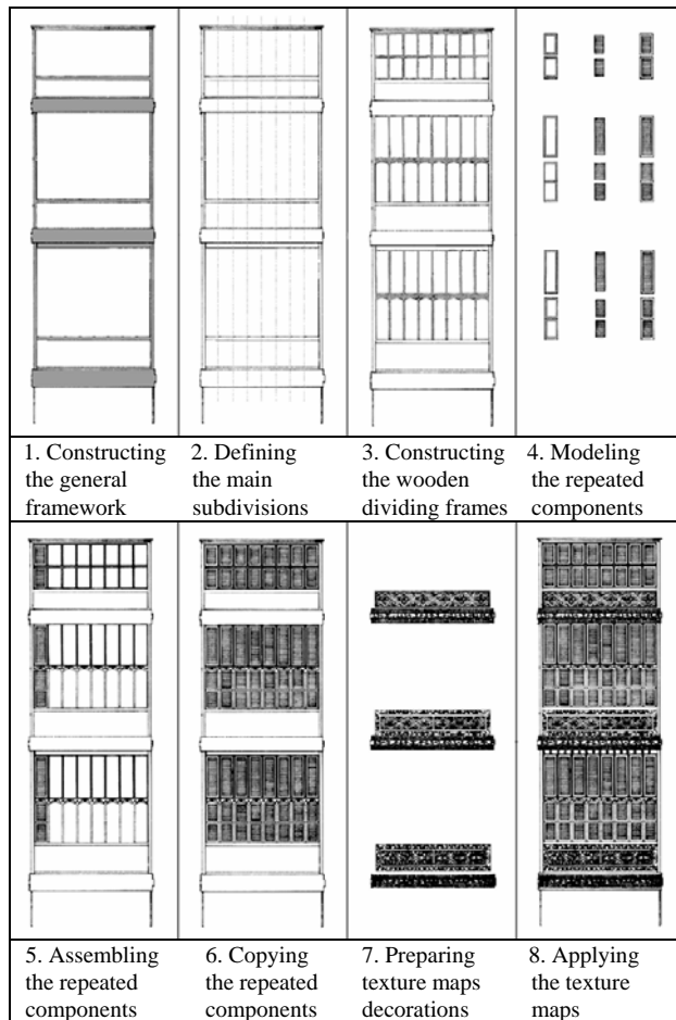
Figure 7. Step 3: Matching the construction process of the elements ( Roshan Example )
