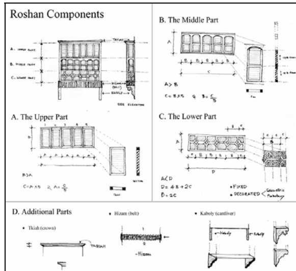
Figure 2. Roshan components and details
